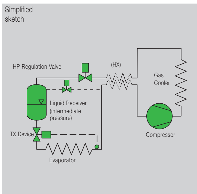
Fig. 31 Example of a transcritical CO 2 system
