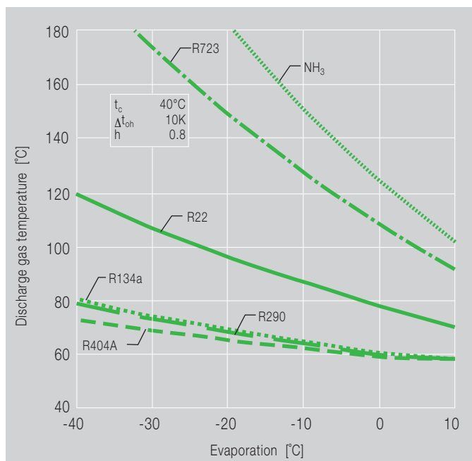
Fig. 25 Comparison of discharge gas temperatures
