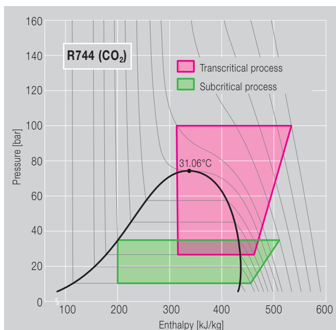
Fig. 29/1 R744(CO 2 ) – pressure-/enthalpy-diagram
