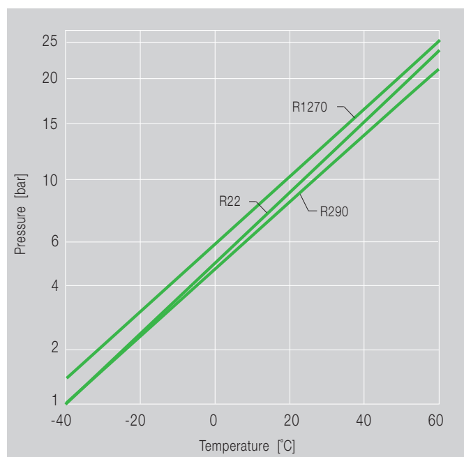
Fig. 28 R290/R1270/R22 – comparison of pressure levels
